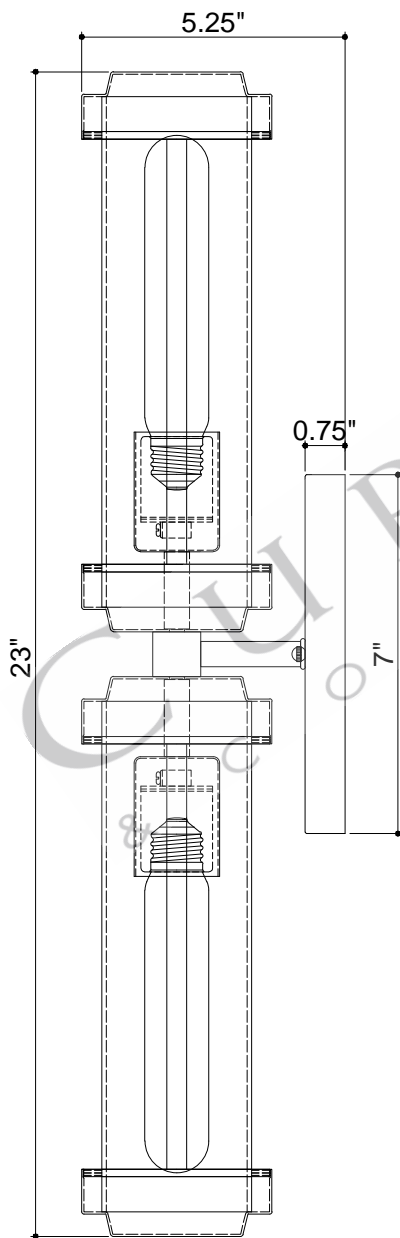
SIDE VIEW
