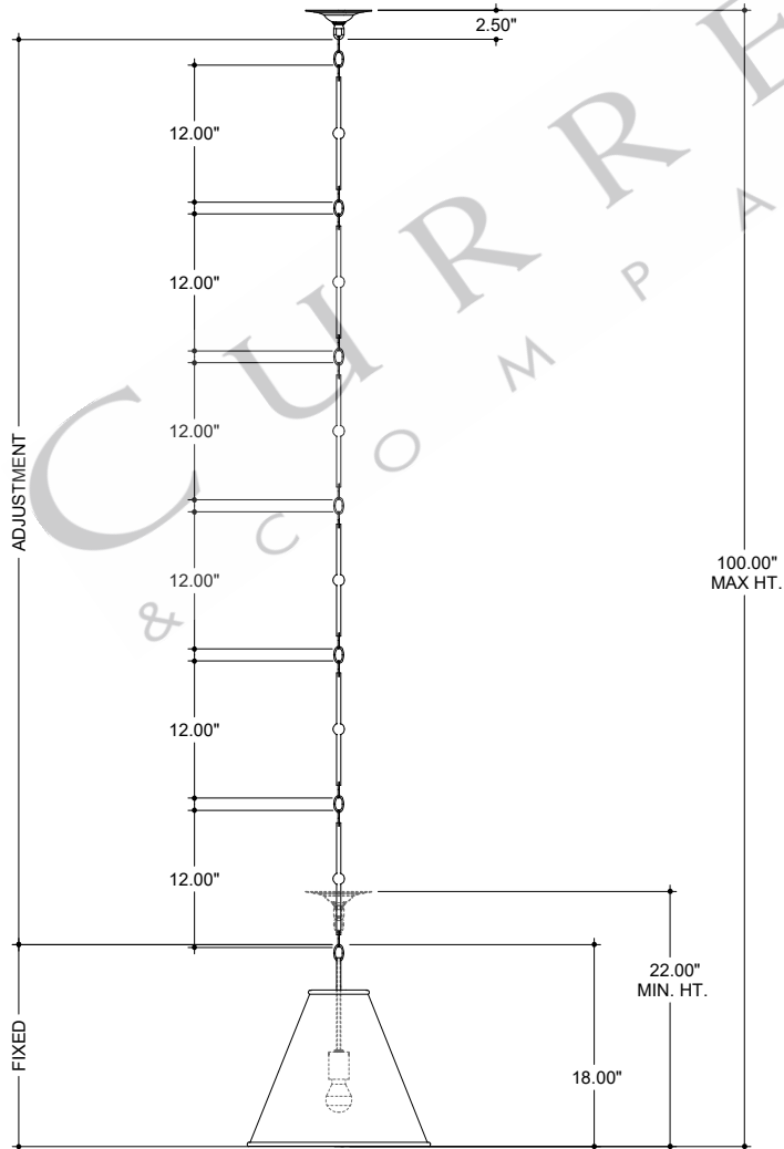
FRONT VIEW
