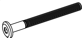
ALLEN KEY BOLT M8 X 70 mm QTY 8
