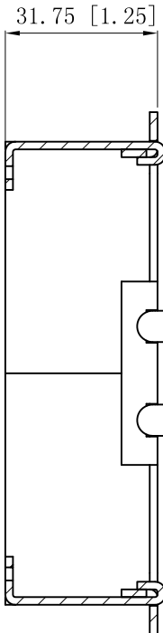
CUTAWAY VIEW A-A
