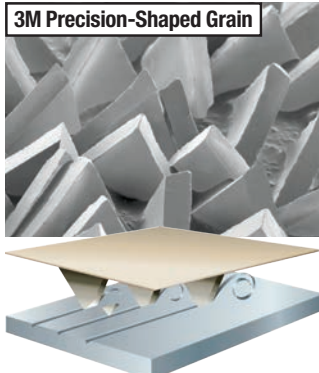
3M Precision-Shaped Grain
