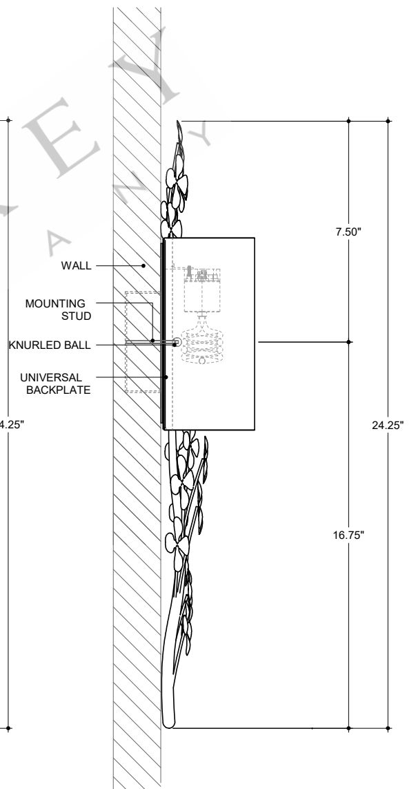
SIDE VIEW
