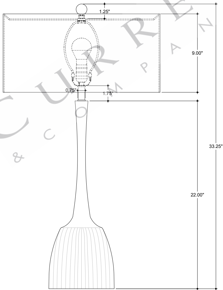
FRONT VIEW
