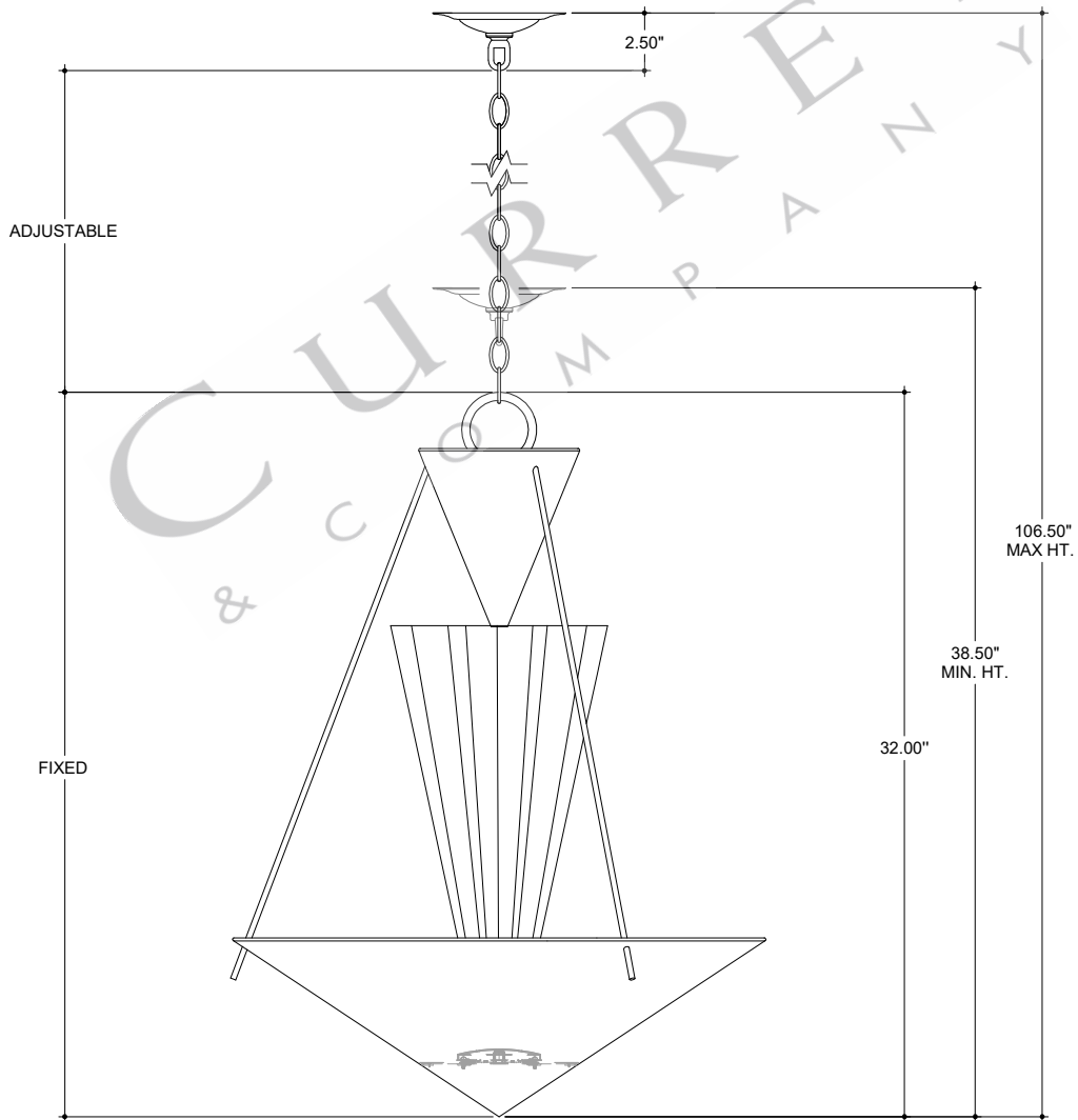
FRONT VIEW
