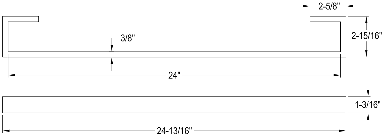
24" Towel Bar
