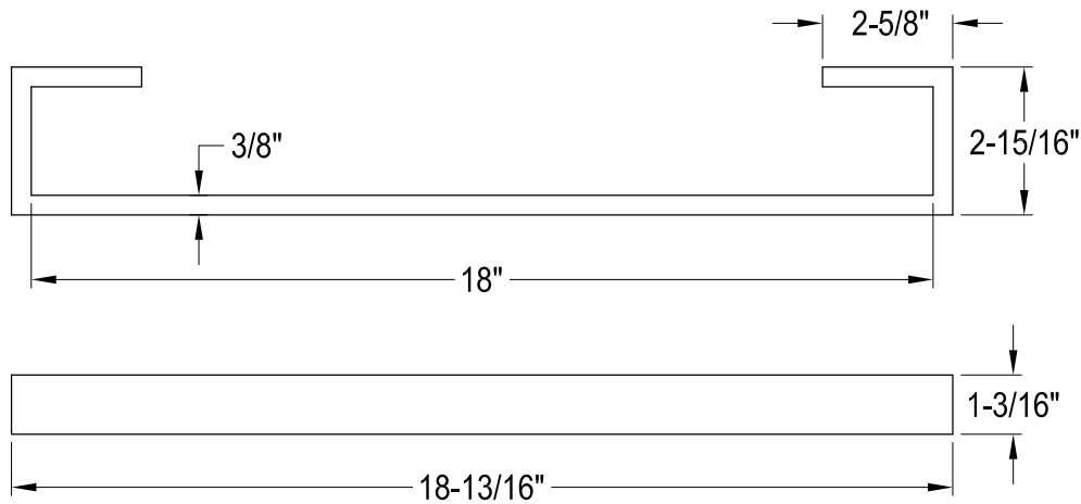
18" Towel Bar
