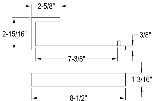
Towel Ring
