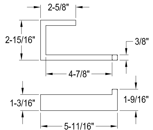
Paper Holder
