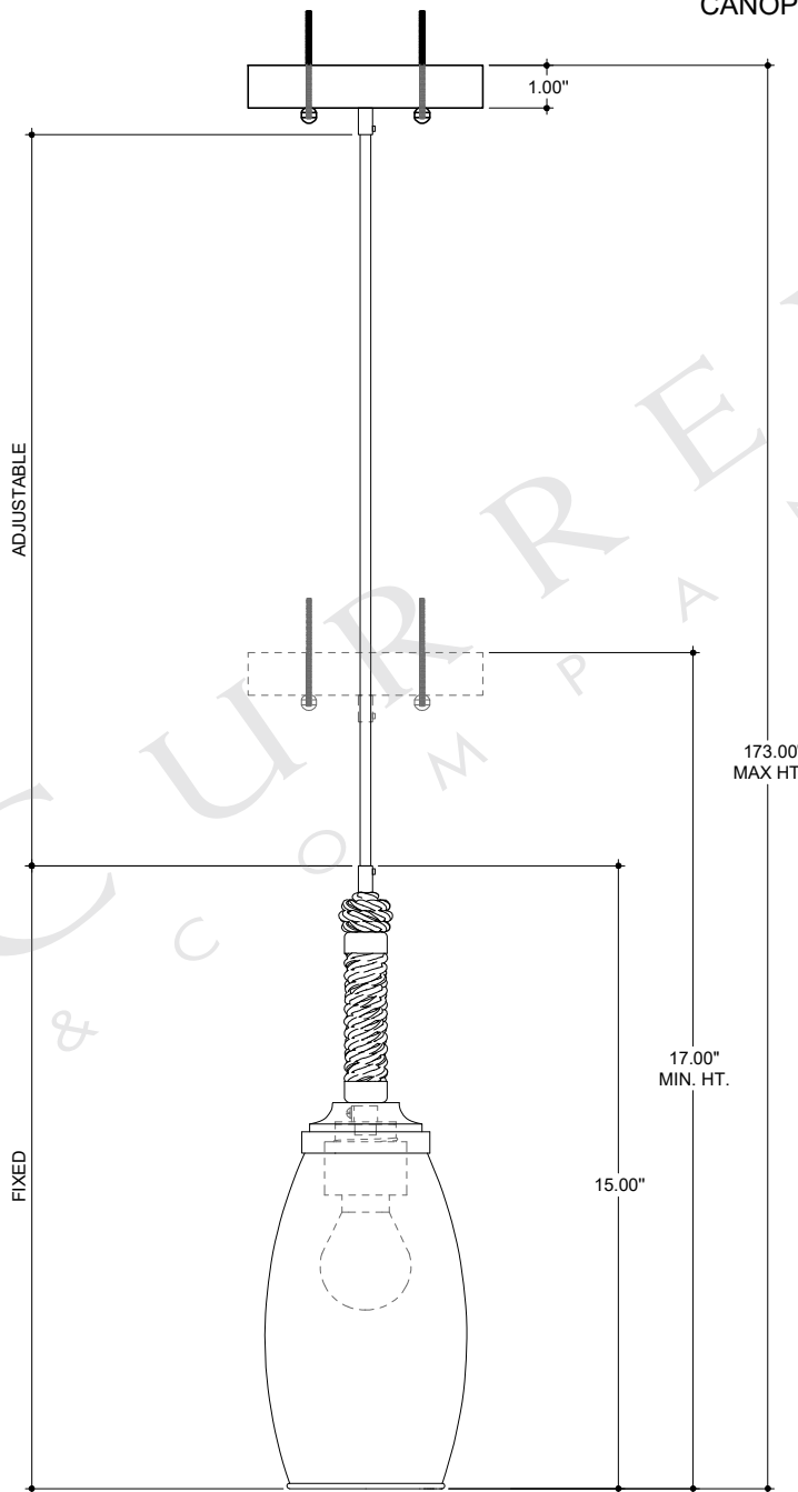
FRONT VIEW
