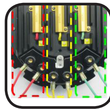
Wire the terminals as shown, use shrink tubing color as a guide
