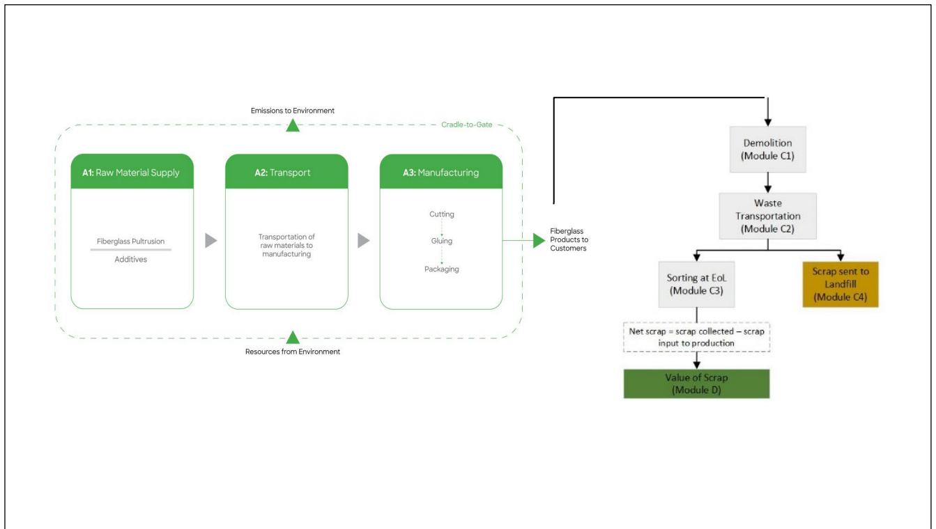
Figure 2 System boundary of the life cycle assessment for Framing Fiberglass product
