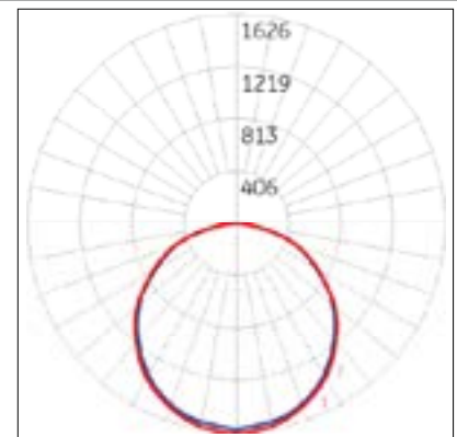
Maximum Candela = 1.963 Located At Horizontal Angle = 260, Vertical Angle = 3 #1 - Vertical Plane Through Horizontal Angles (260 - 80) (Through Max. Cd.)
