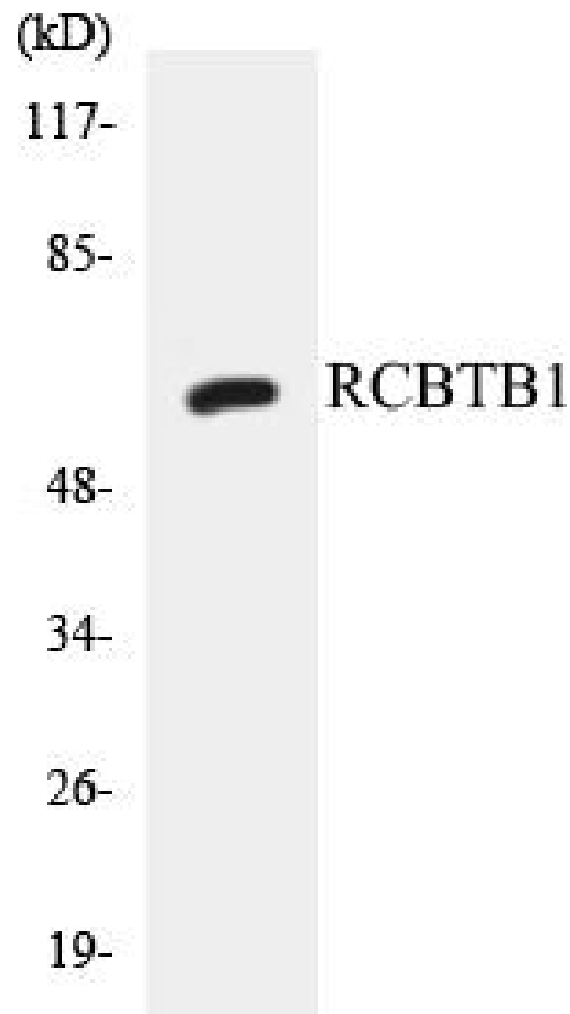
Figure 2. Western blot analysis of extracts from LOVO cells, using RCBTB1 Antibody.
