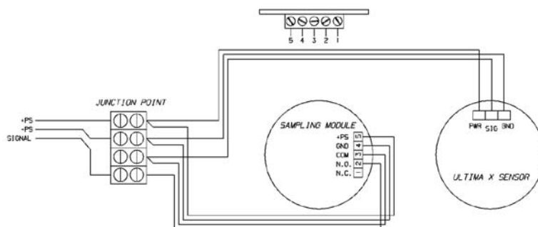
Figure 2-2. Typical Wiring
