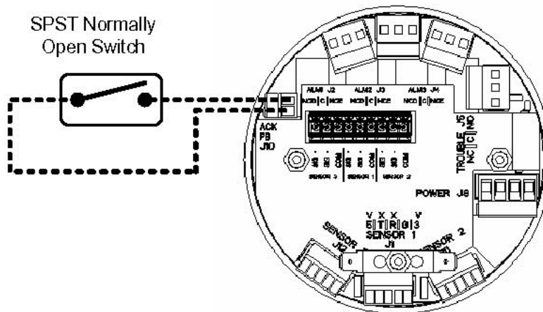
Figure 2-4. Push-button Wiring
