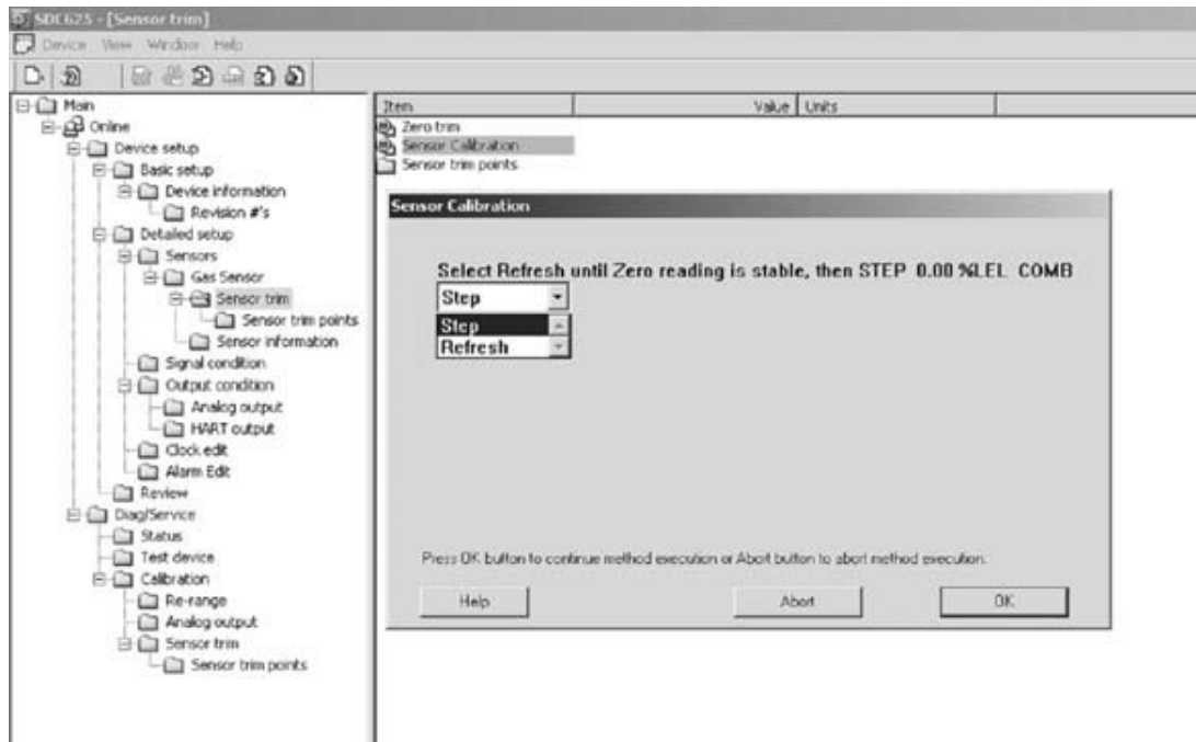
Fig. 33 Zero cal step screen
