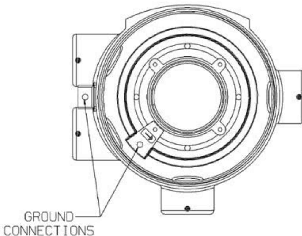
Fig. 11 Ultima XE Grounding Terminals
