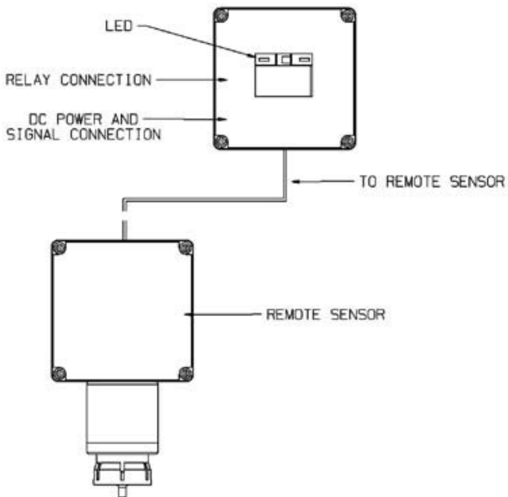
Fig. 20 Remote Module General-Purpose Ultima X Series Wiring
