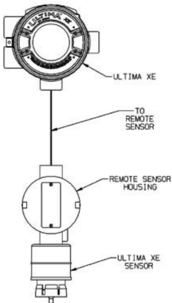
Fig. 21 Remote Module Explosion-Proof Ultima X Series Wiring
