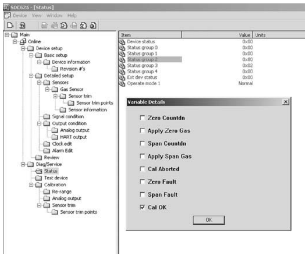
Fig. 48 Calibration status screen
