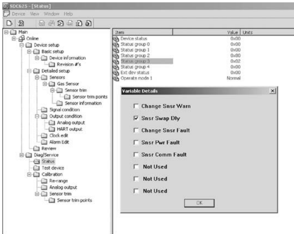
Fig. 50 Additional Sensor Status screen
