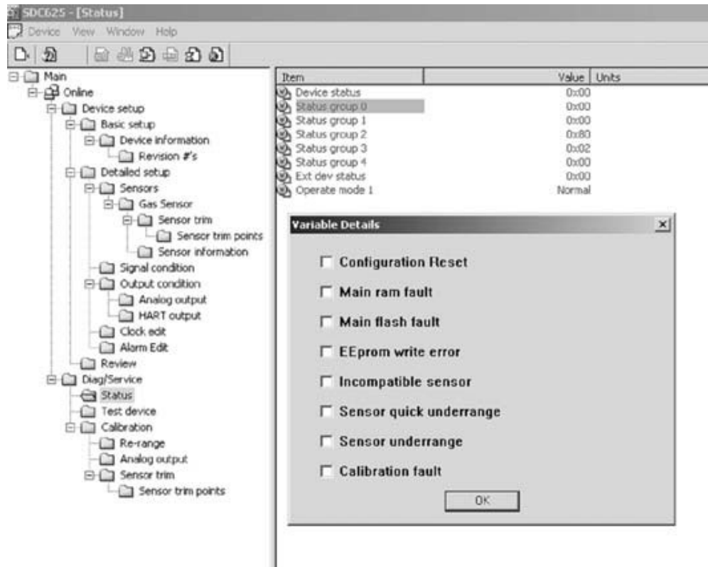
Fig. 51 Device Status screen
