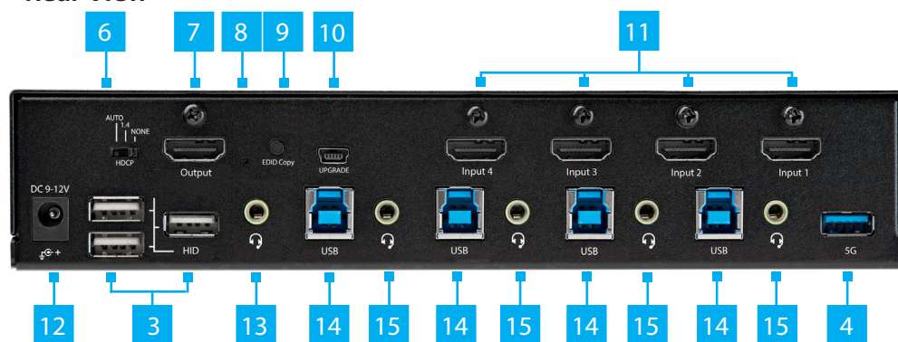
Rear View
