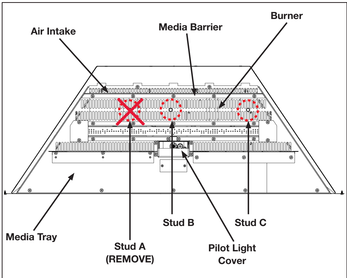
Burner Overview
