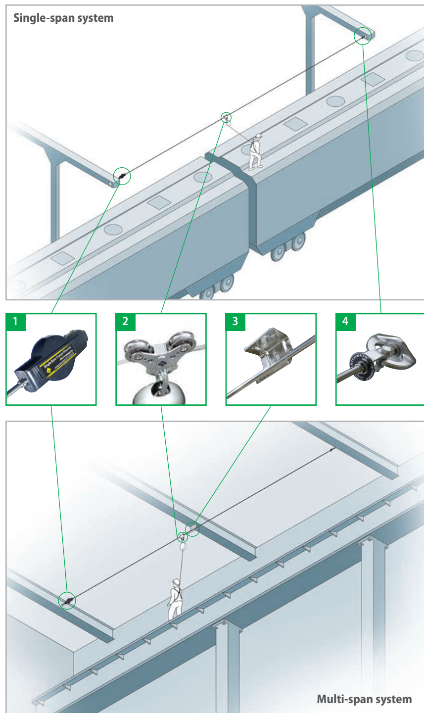
Typical uses of overhead systems illustrated: rail car loading bay (top) and internal factory access (below).
