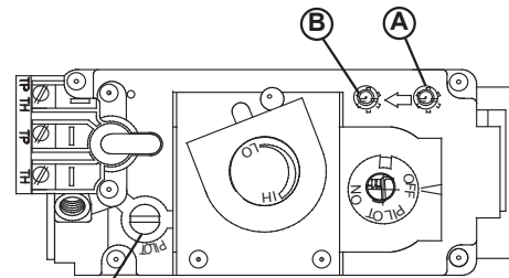
PILOT SCREW
