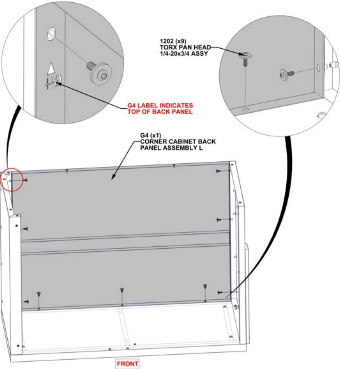
G4 CORNER CABINET BACK PANEL ASSEMBLY L - A4M03033 (x1) 1 3/16"x33 3/8"x47 13/16" (30x848x1215)
