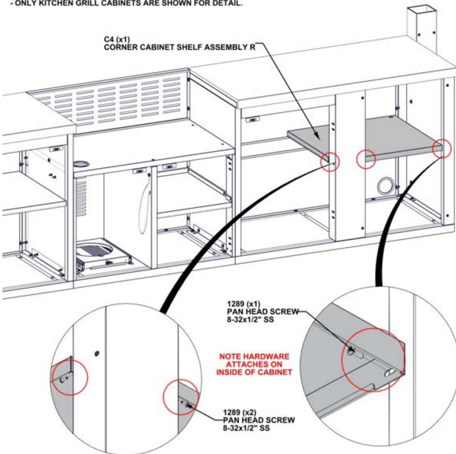
C4 CORNER CABINET SHELF ASSEMBLY R - A4M03046 (x1) 1 1/4"x23 1/8"x25 7/16" (32x588x646)
