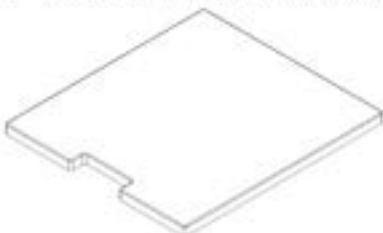
M3 PIZZA OVEN CABINET MARBLE R - A4M03090 (x1) 1 15/16"x20"x24 13/16" (50x508x630)
