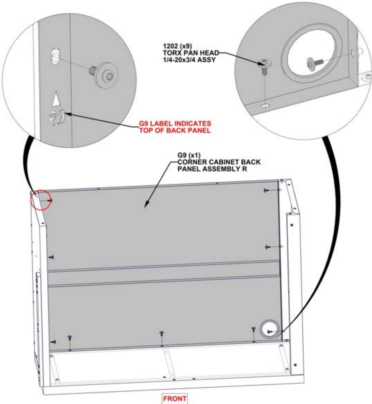
G9 CORNER CABINET BACK PANEL ASSEMBLY R - A4M03043 (x1) 1 3/16"x33 3/8"x47 13/16" (30x848x1215)
