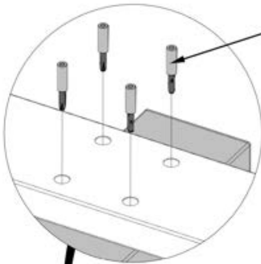
1103 (x4) TORX SOCKET SCREW 1/4-20
