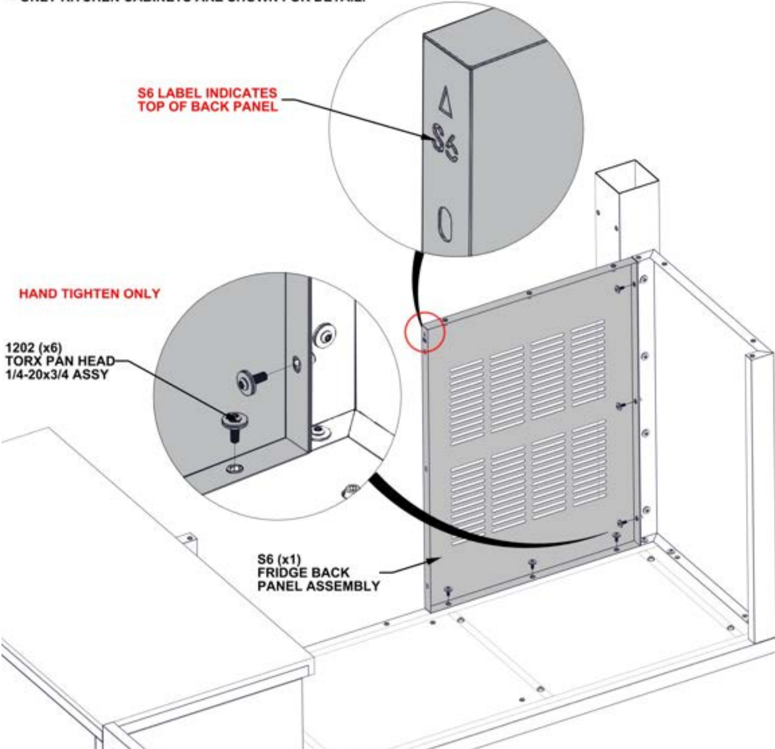
S6 FRIDGE BACK PANEL ASSEMBLY - A4M03099 (x1) 1 3/16"x24 1/2"x33 3/8" (30x623x848)
