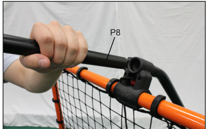
STEP 4: Remove Upper Boom Tube P8 and set aside.
