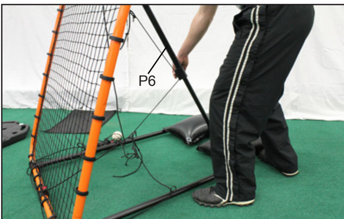
STEP 7: Loosen the knob on Top Back Telescoping Tube P6 and adjust rebounder to desired angle.
