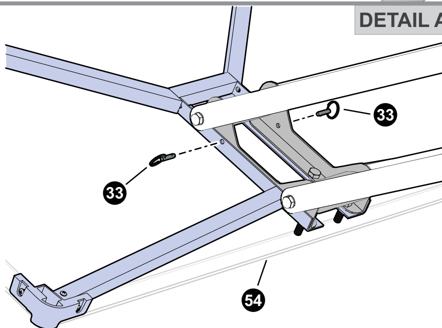
DETAIL B
