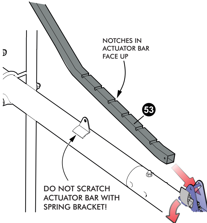
DETAIL A
