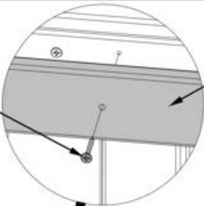
387 (x7) SCREW - 1 1/4"
