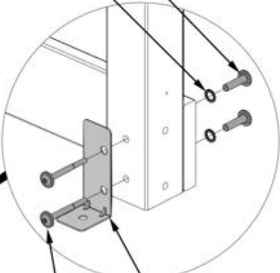
2503 (x1) ANCHOR BRACKET
