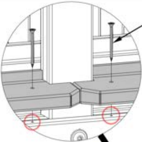
391 (x15) SCREW - 2"
