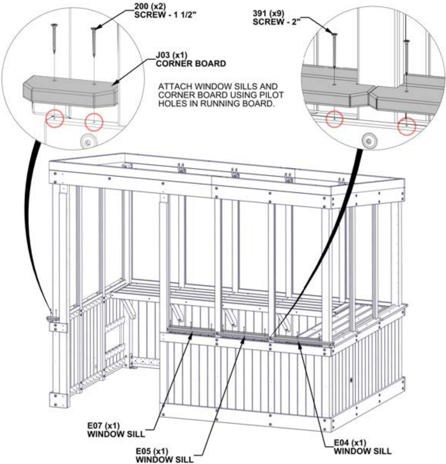
E05 WINDOW SILL - W4L19197 (x1) 1 7/16"x3 3/8"x21 5/16" (36x86x542)
