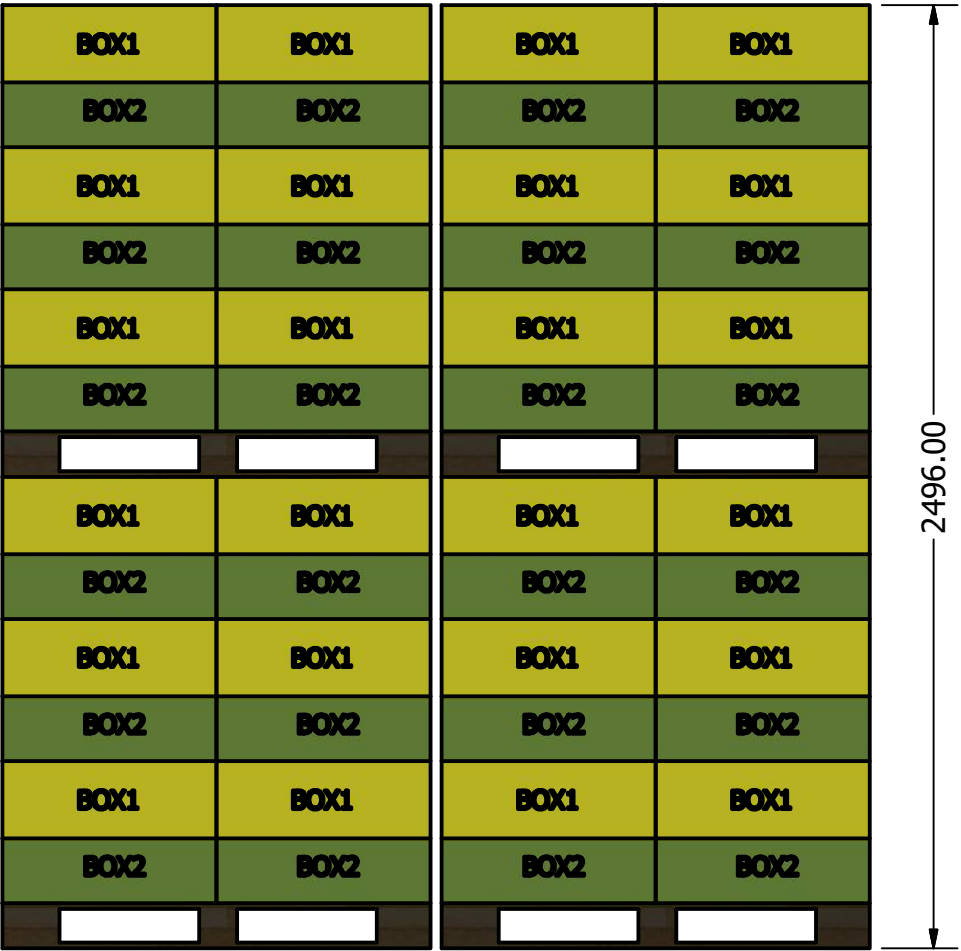
End view
