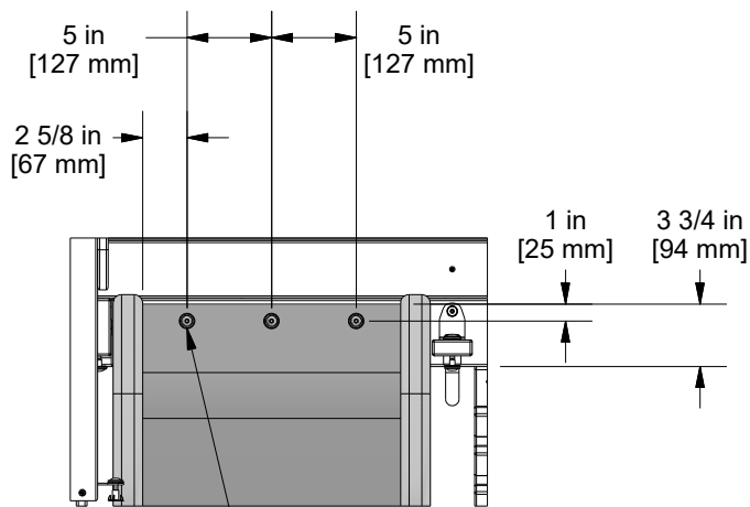
SLIDE ASSEMBLY
