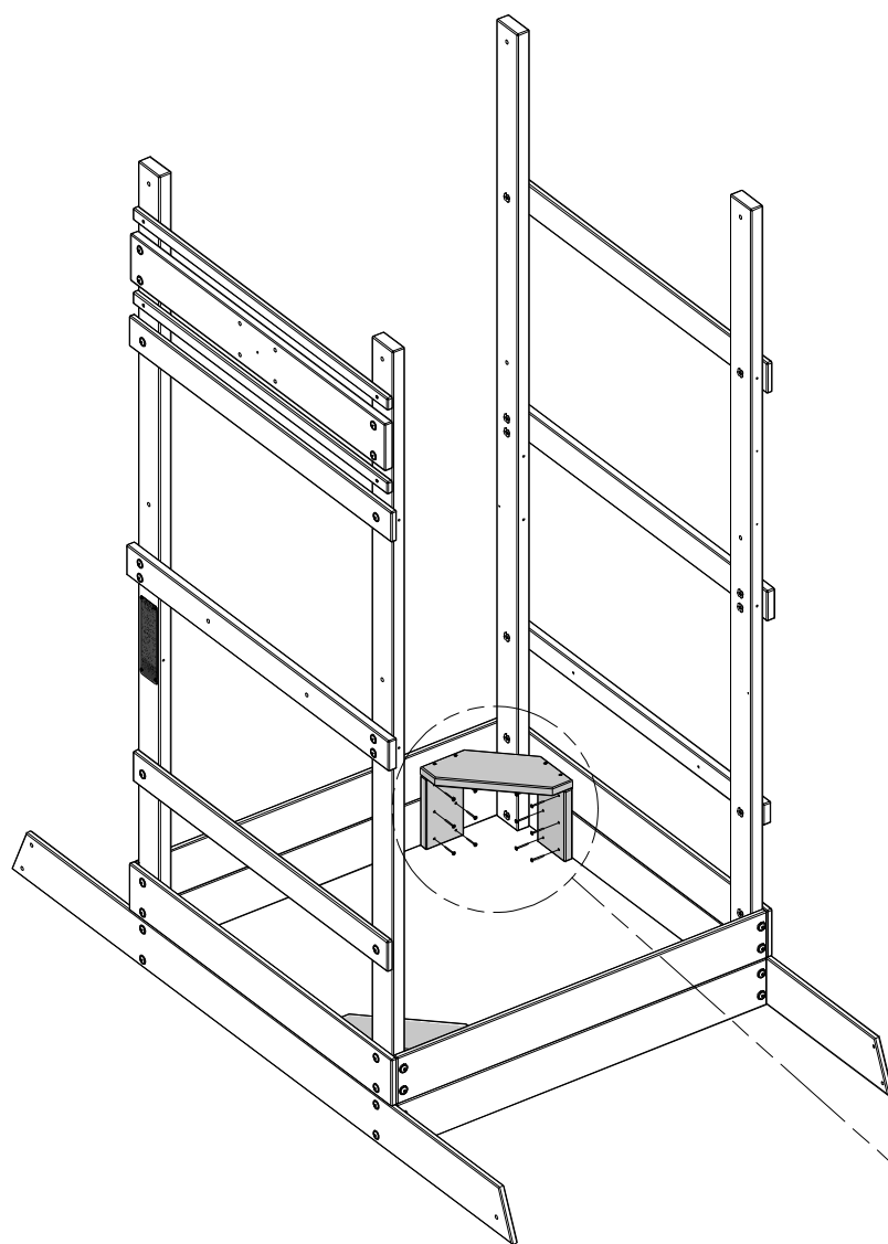
089 (x8) SCREW - 1 3/4"
