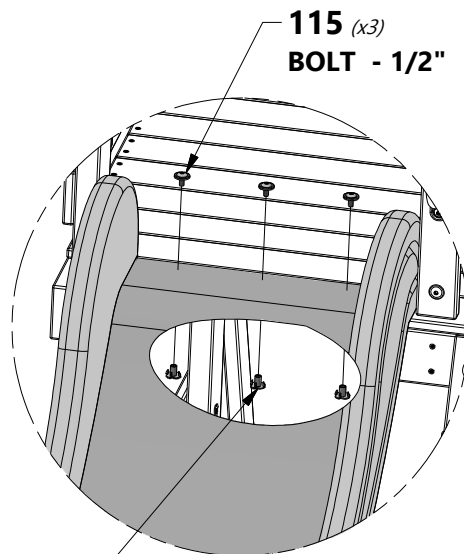
074 (x3) T-NUT - 5/16"
