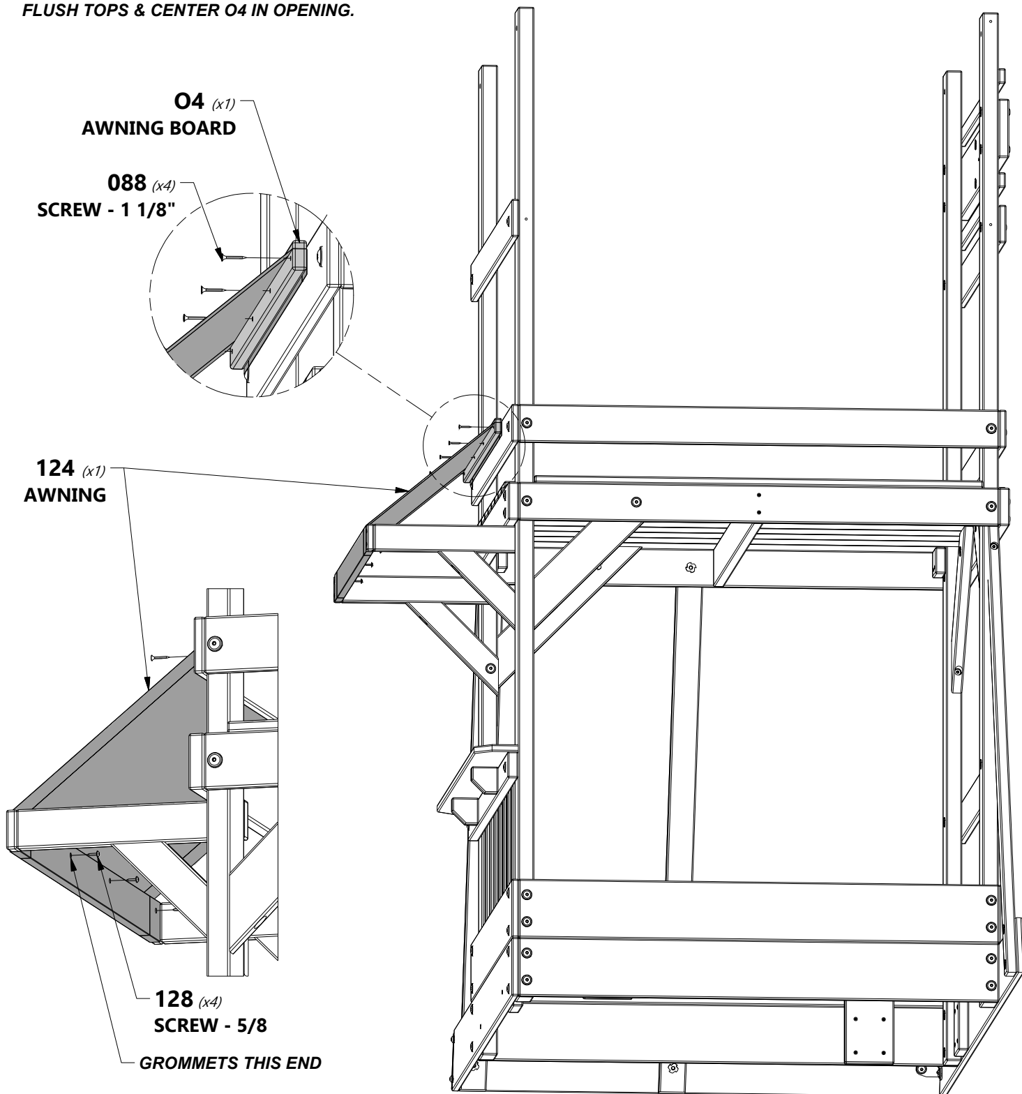
A6P00124 | AWNING (1)
