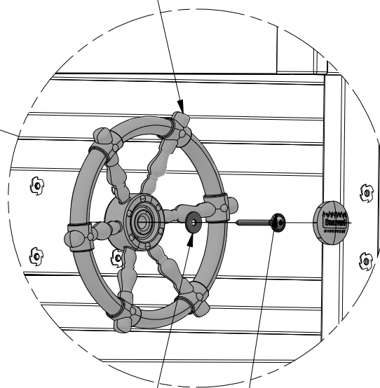
105 (x1) WASHER - 8x27 029 (x1) LAG SCREW - 3"
