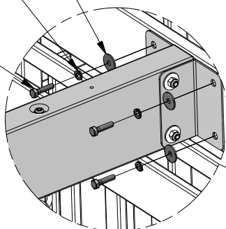
095 (x4) | WASHER - 5/16"
