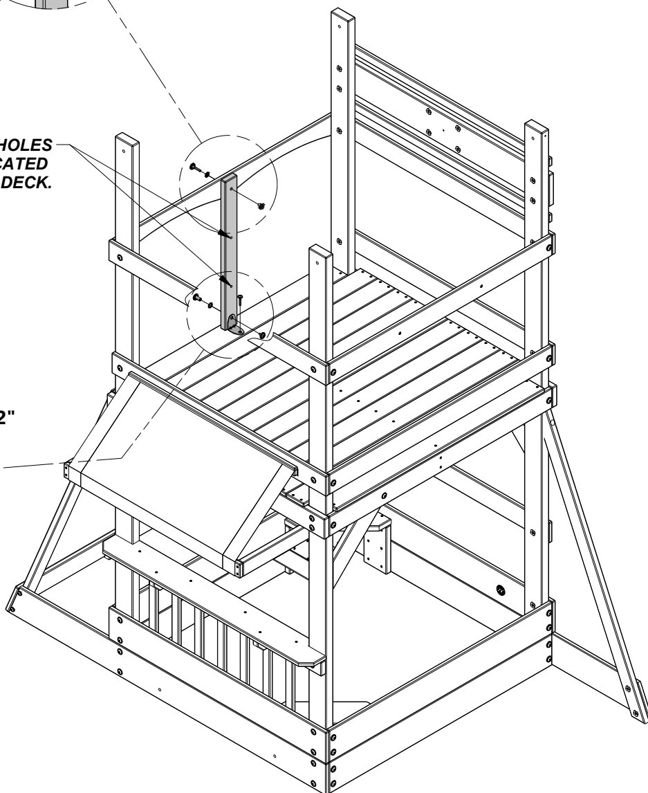
048 (x1) L BRACKET 2.5x38x55x55
