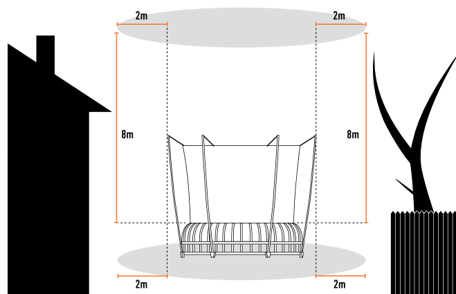
Correct Installation
