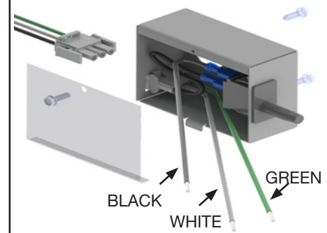
FIGURE 28 - ELECTRICAL CONNECTIONS / MOLEX CONNECTOR
