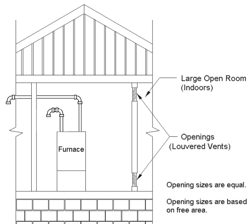
FIGURE 4 - COMBUSTION/DILUTION AIR FROM HEATED INSIDE SOURCES (CASE 2)
