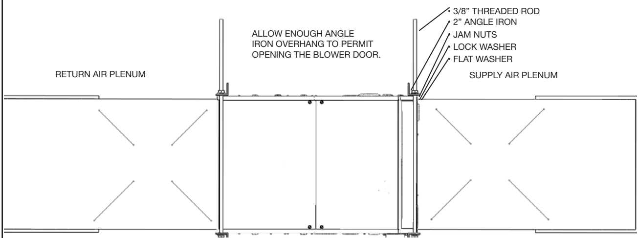
FIGURE 3 - SUGGESTED METHOD FOR SUSPENDING HORIZONTAL FURNACE
