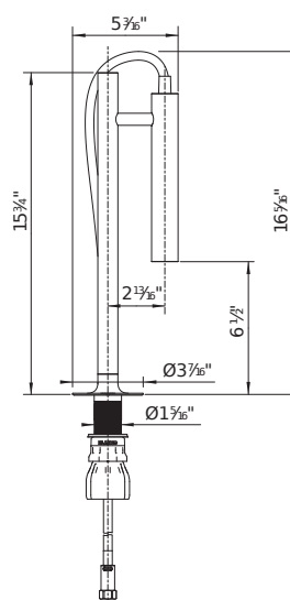
Side view lever
