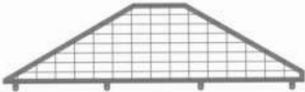
7061 MESH PANEL - A4M07061 (x1) 2 1/16"x18 1/8"x62 5/16" (53.0x459.9x1582.4)
