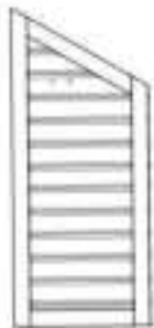
WP4 WALL PANEL - W2A04943 (x1) 1 1/8"X19 1/16"X44 9/16" (27X484X1133)
