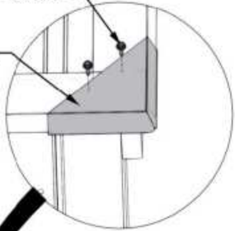
1116 (x4) SCREW SELF TAPPING
