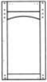
WP9 DOOR FRAME - W2A04951 (x1) 1 7/16"X18 13/16"X33 1/2" (36x478x650)
