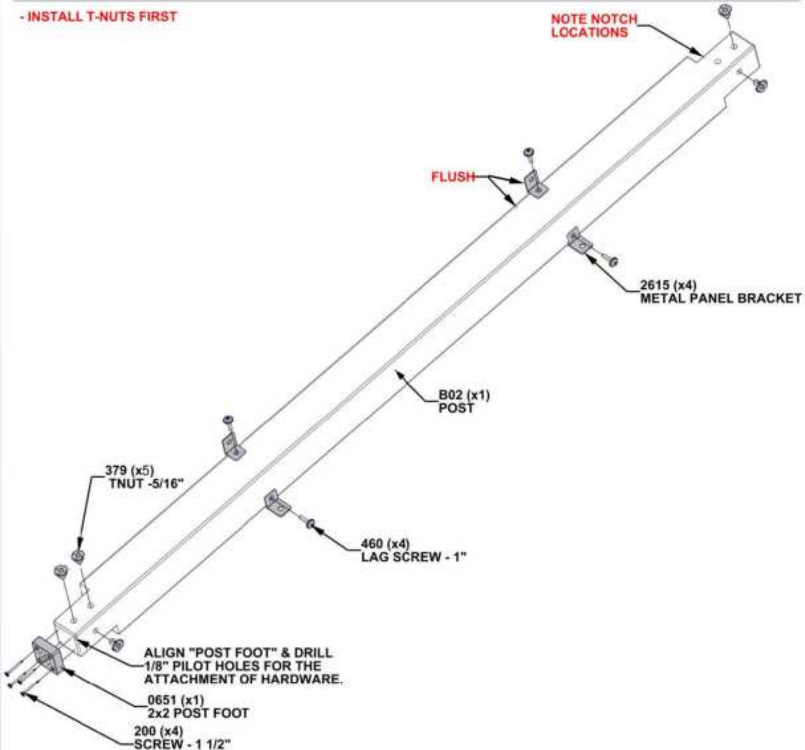
A6P00651 2x2 POST FOOT (x1)
