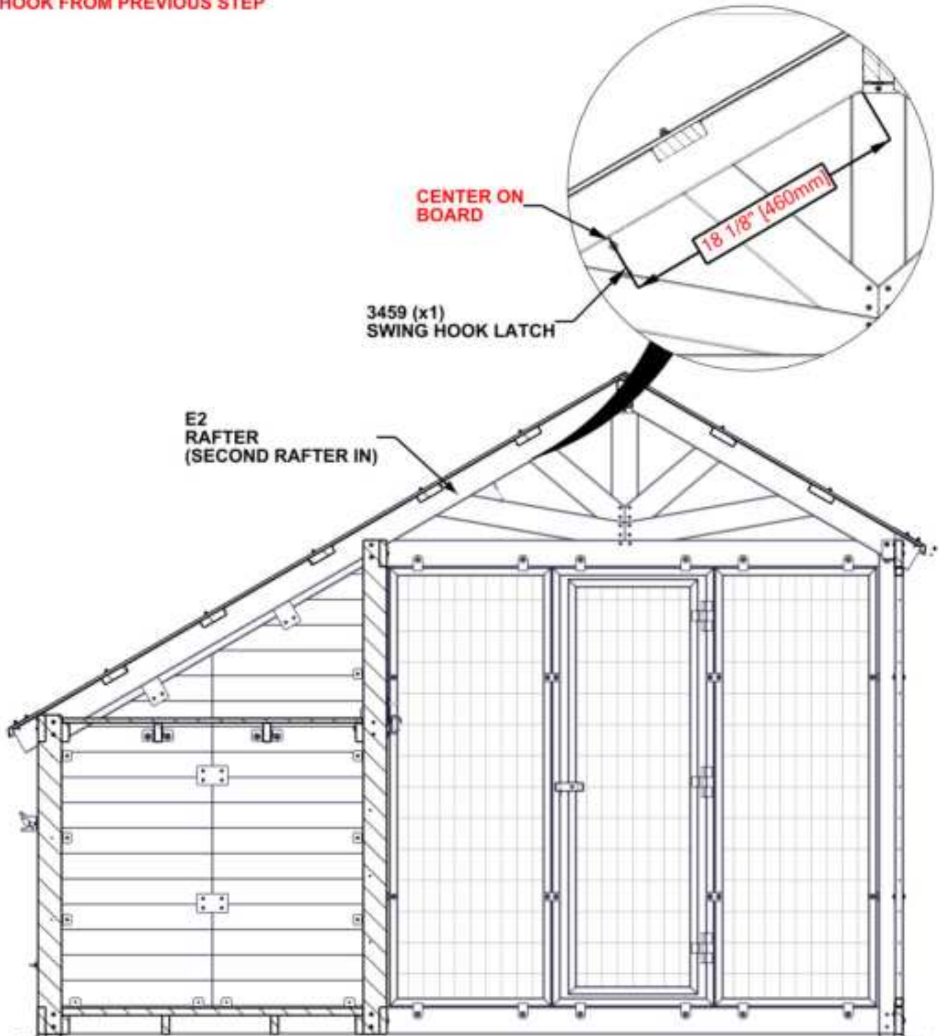
A4M03459 SWING HOOK LATCH (x1)
