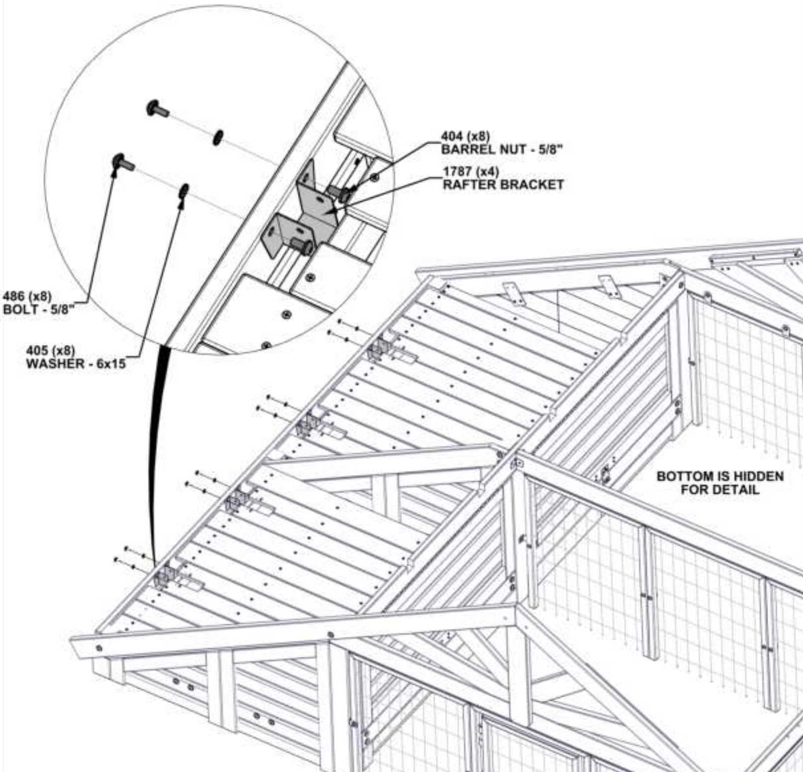
A4M01787 RAFTER BRACKET (x4)
