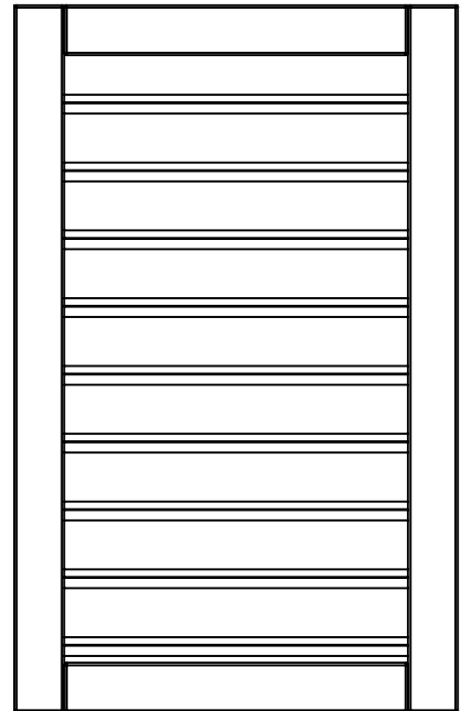
WP10 WALL PANEL-W2A04952 (x1) 1 1/16"X21"X33 1/2" (27x534x850)
