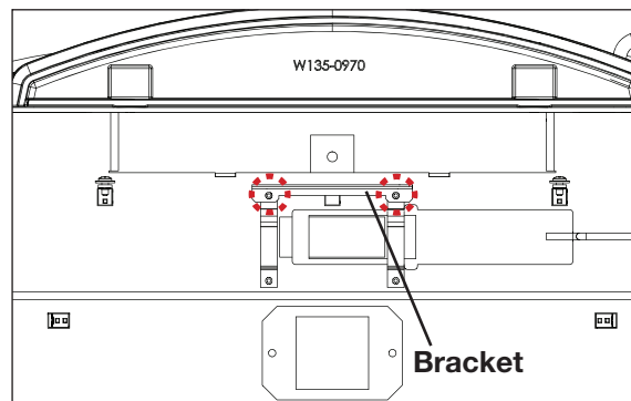
Bottom view of appliance (some components hidden for clarity)
