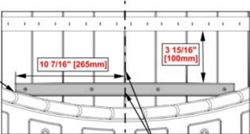
CENTER SEAM AND CENTER BOARD
