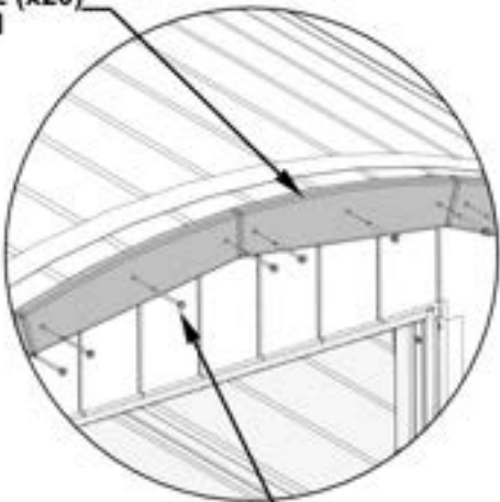
1429 (x60) SCREW - 2"
