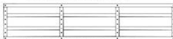
BR02 BENCH BACK REST - W2A04791 (x2) 1 15/16"x12 1/16"x55 7/16" (50x306x1408)
