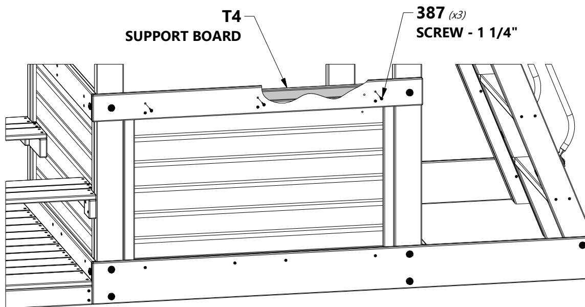
OUTSIDE VIEW
