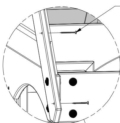
089 (x8) SCREW - 1 3/4"
