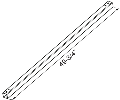
P7B - 3 pcs - Bottom Back Rebounder Beam (1 pc) - Goal Net Support Beam (2 pcs)
