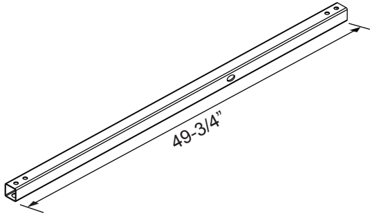
P12 - Left & Right Back Rebounder Side Beam (2 pcs)
