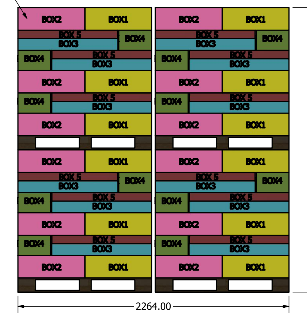
End view
