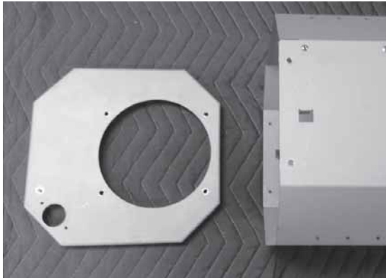
1. Remove internal blower flange from motor housing by (6) screws.
