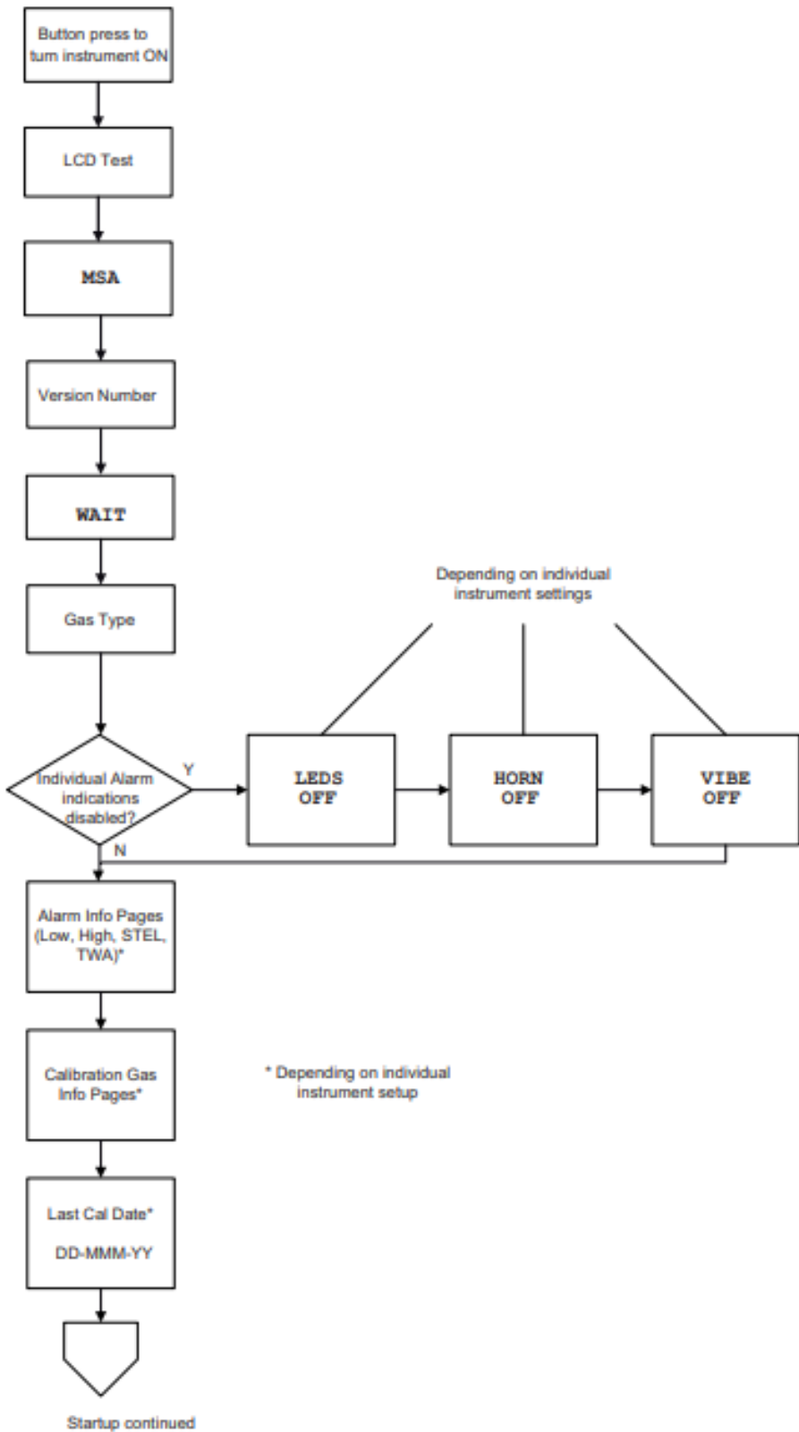
Figure 3 Startup
