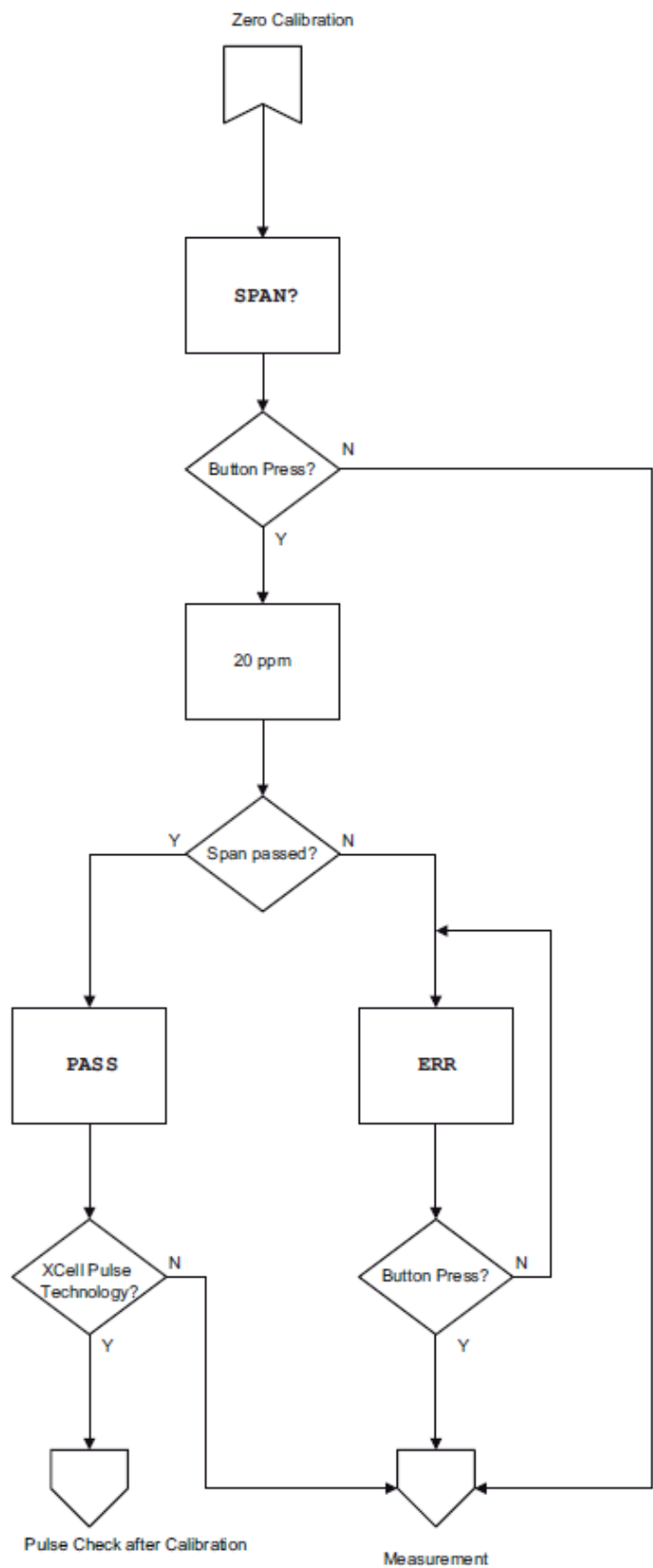
Figure 12 Span calibration
