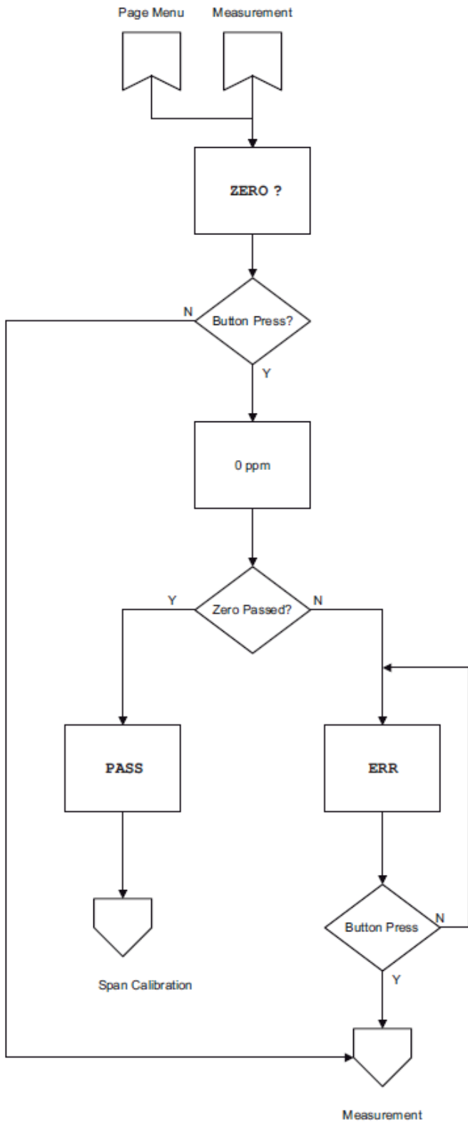
Figure 11 Zero calibration
