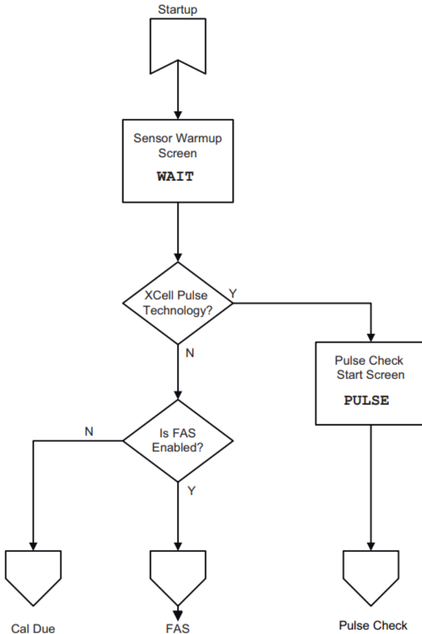
Figure 4 Startup, continued
