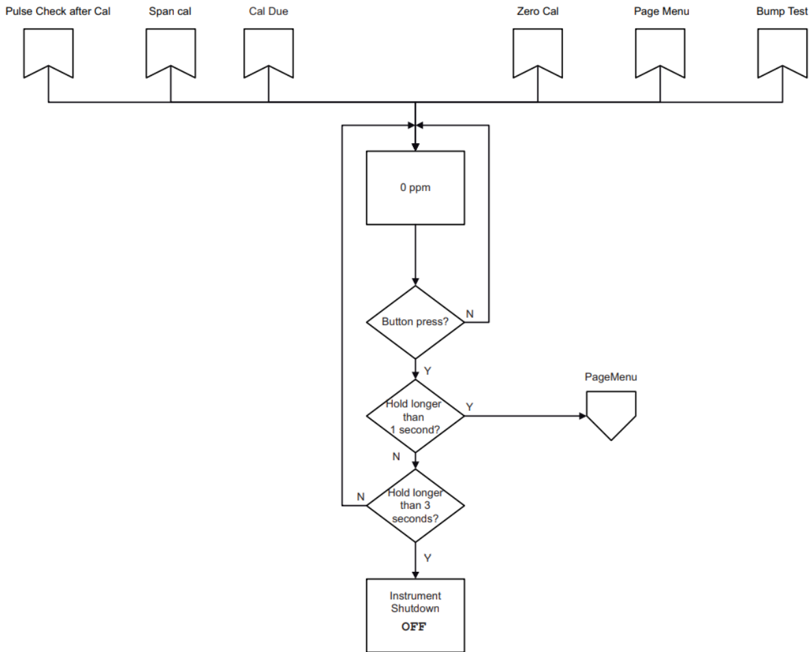
Figure 8 Measurement
