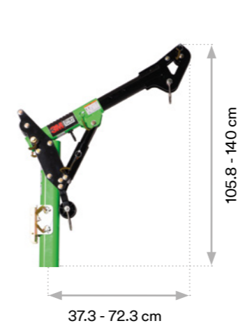
3M™ DBI-SALA® Short Reach Davit Arm High Capacity (14" - 28")
