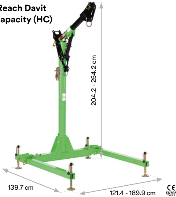
3M™ DBI-SALA® 5 Piece Long Reach Davit High Capacity (HC)
