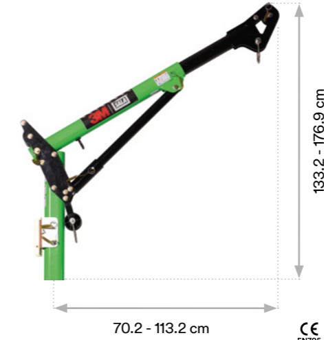
3M™ DBI-SALA® Long Reach Davit Arm High Capacity (27" - 44")
