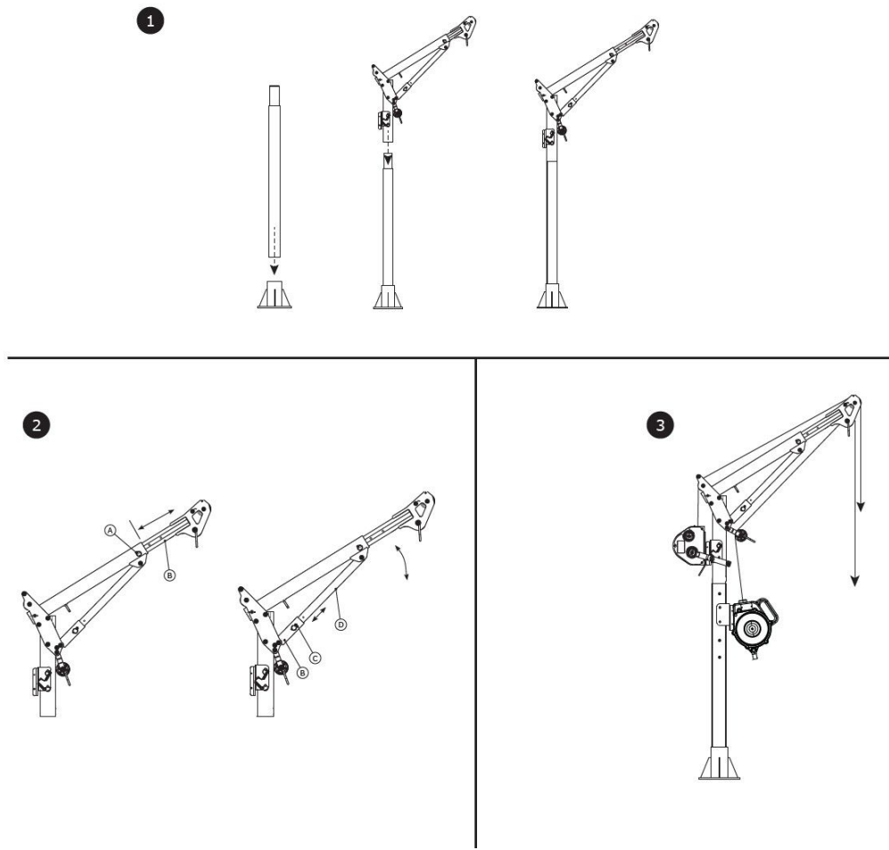
Figure 7 - Installing the Davit System
