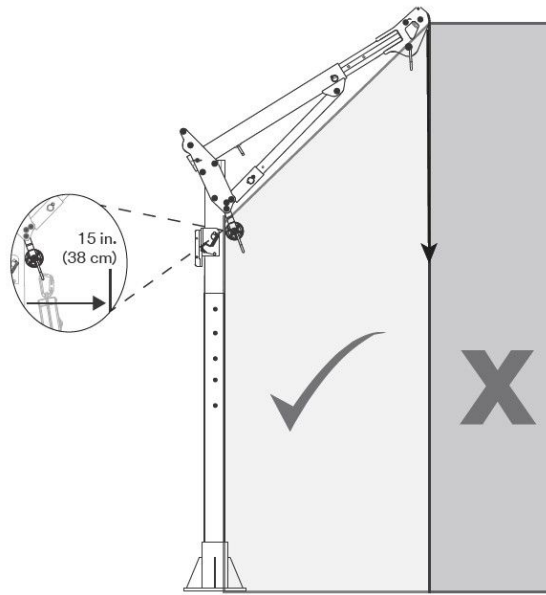
Figure 5 - Safe Working Area
