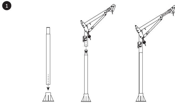
Figur 7 – Montere davitsystemet
