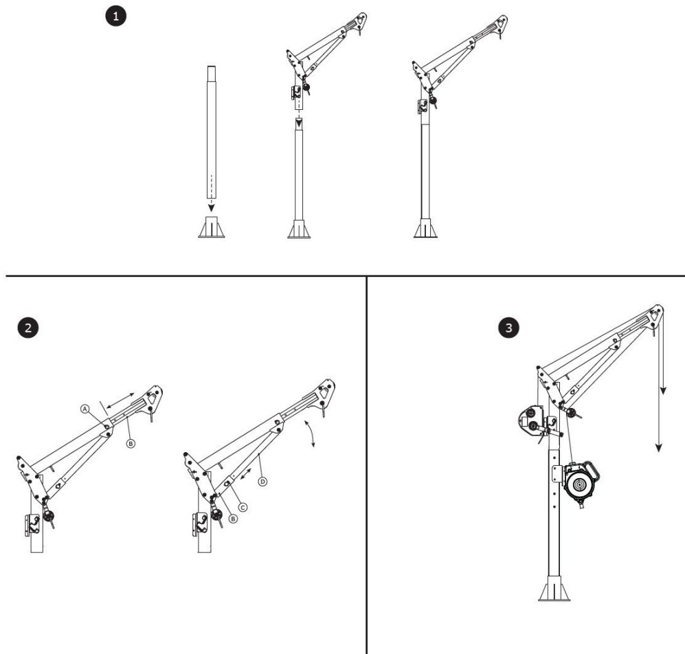
Figur 7 – Installera Davit-systemet
