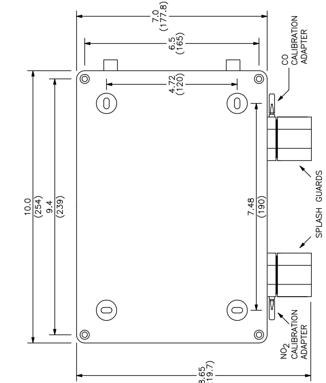
NEMA4X FIBERGLASS ENCLOSURE WITH HINGED SCREW COVER
