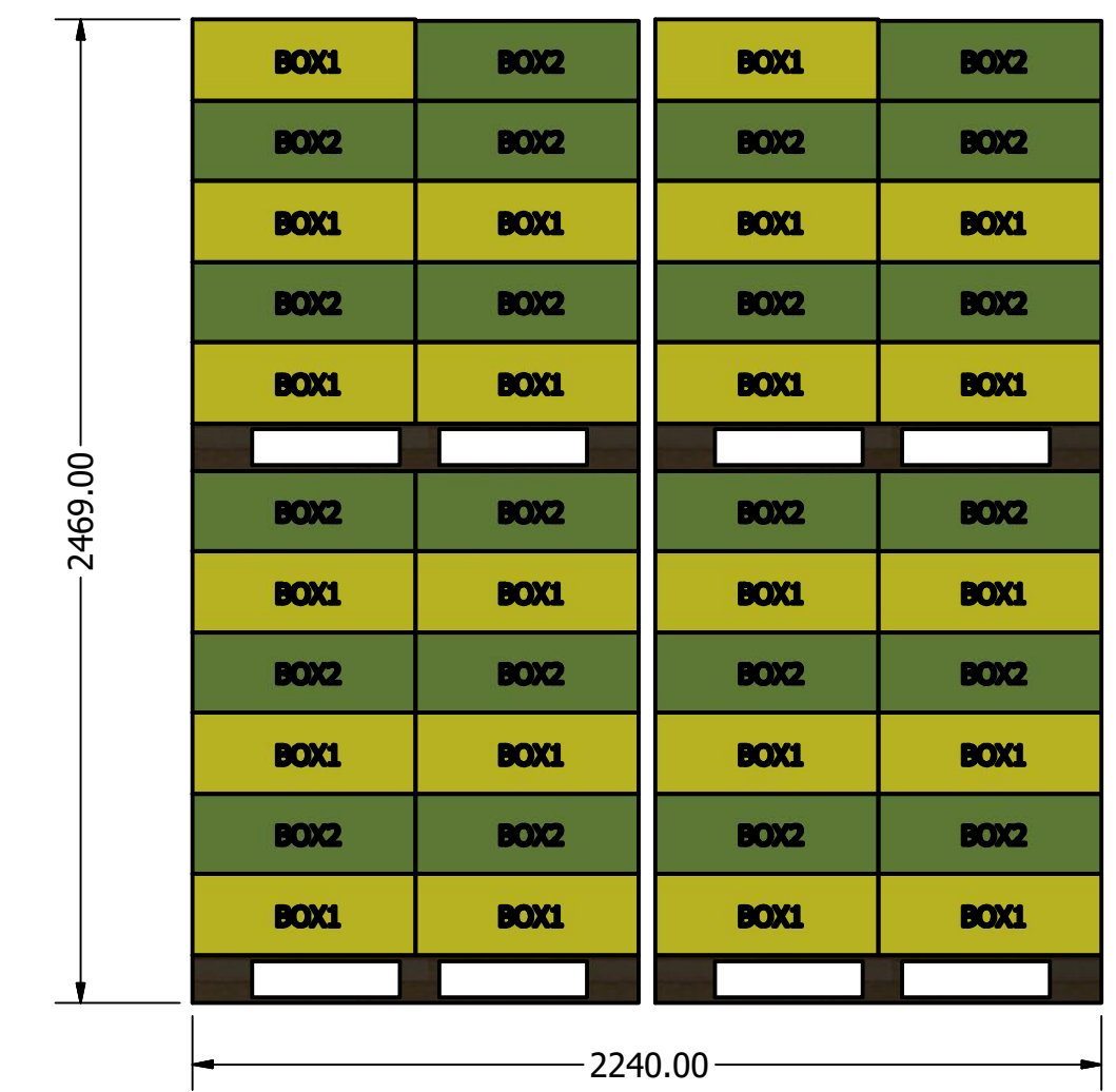
End view
