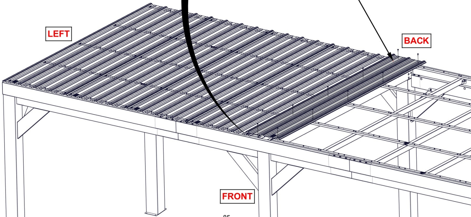
2926 (x1) 29 GA STEEL SHEETING
