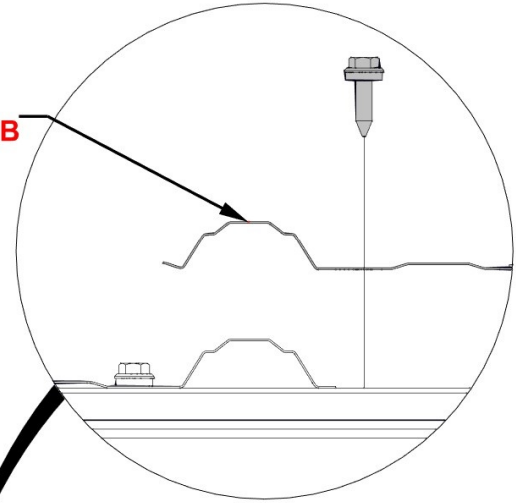
2925 (x3) 29GA STEEL SHEETING
