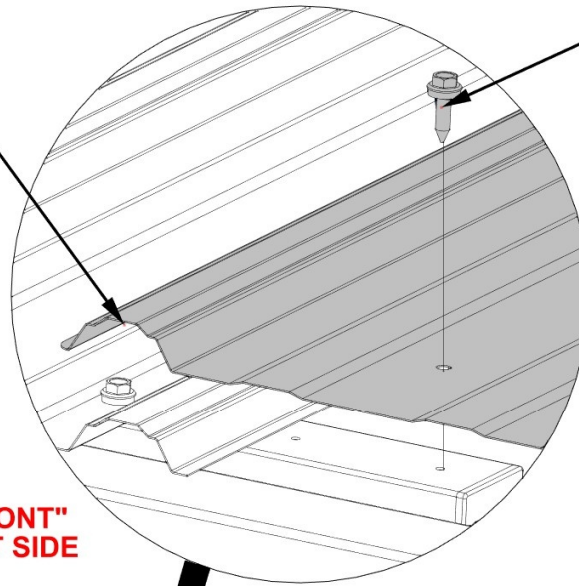
2926 (x1) 29 GA STEEL SHEETING
