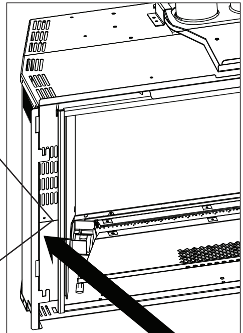
Left side view of appliance (TDIG3 illustrated)
