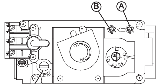
PILOT SCREW
