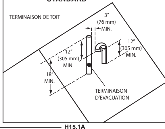
FIGURE 11 - CONFIGURATION D'ÉVACUATION VERTICALE STANDARD
