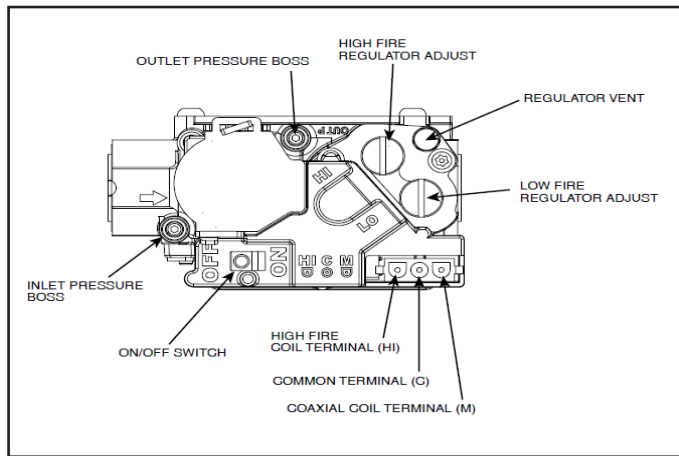
FIGURE 28 - WHITE RODGERS 36G54 GAS VALVE
