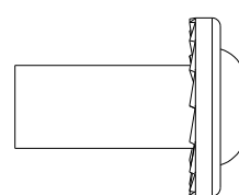
H100192 | NUT BARREL WH BLK (x42) | 5/16x7/8
