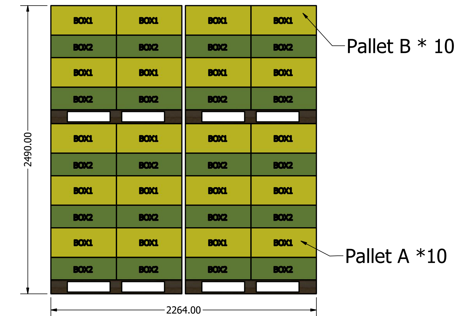
End view
