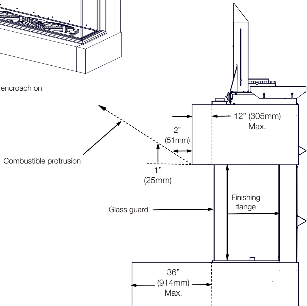
Side View
