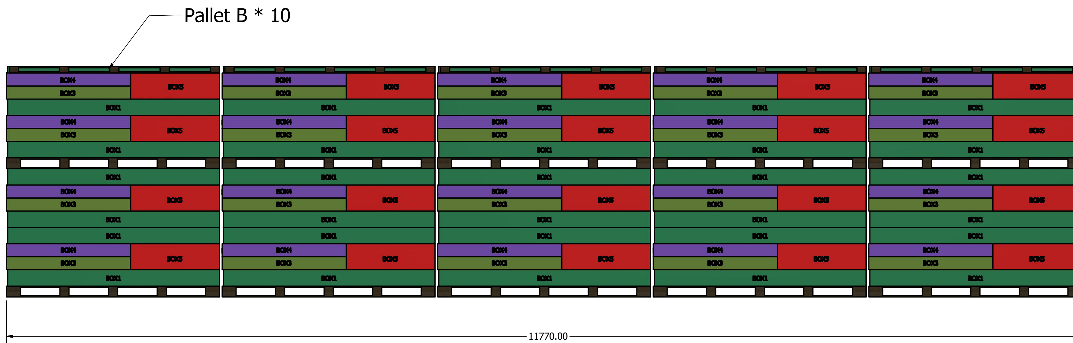
Side view
