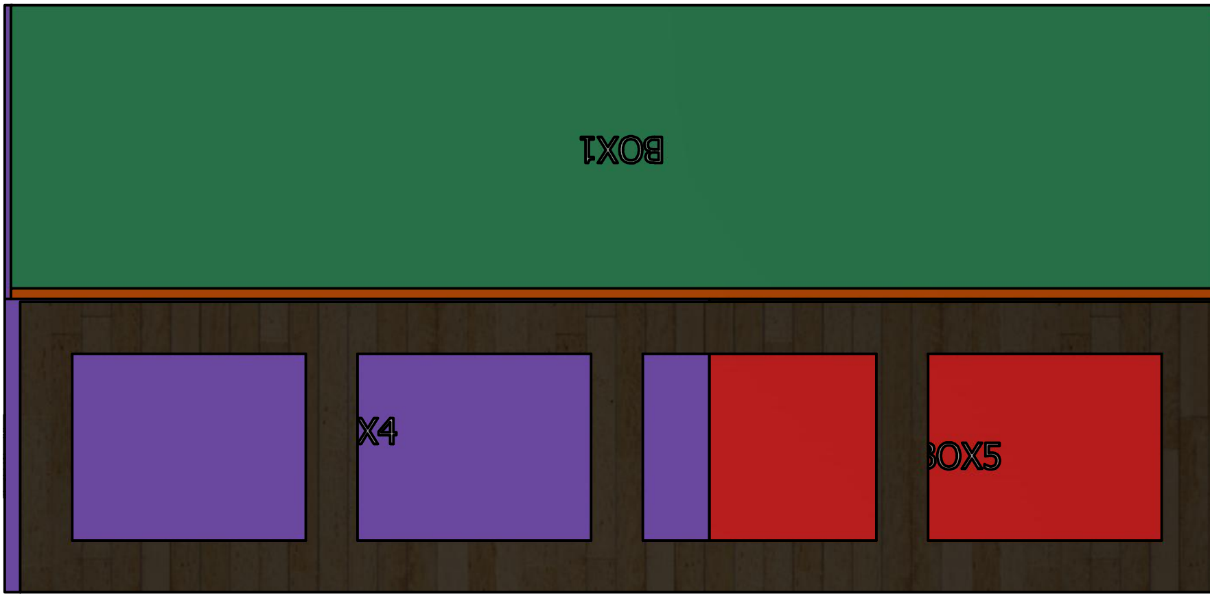
Side View
